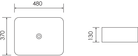
CBH00 Ceramic basin size: 480x370x130 mm
