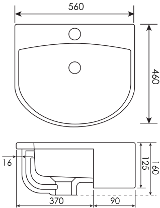
DIONE-56SR Semi-recessed basin Size: 560x460x160mm
