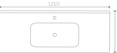
MONZA46 120 SIZE: 1210X465X170 MM
