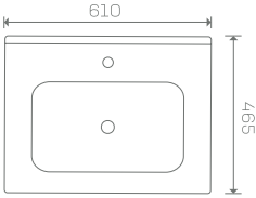
MONZA46 60 SIZE: 610X465X170 MM
