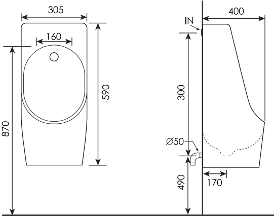
URINAL-01 Wall-hung Urinal Size: 305x400x590mm Drain: Wall drainage or Direct drainage Water Intake: Back
