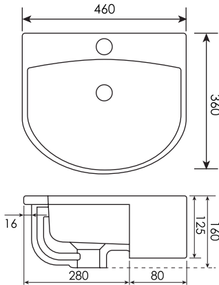
DIONE-46SR Semi-recessed basin Size: 460x360x160mm
