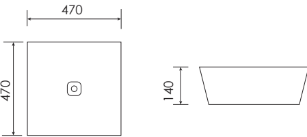
CBHTC Ceramic basin size: 470x470x140 mm
