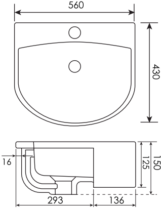
GLIDE-56SR Semi-recessed basin Size: 560x430x150mm
