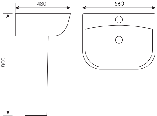
GLIDE-56SP Pedestal basin Size: 560x480x800mm
