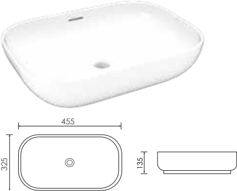
CBCLTA-O Ceramic basin size: 455x325x135mm
