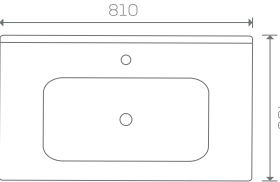
MONZA46 80 SIZE: 810X465X170 MM
