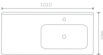
MONZA46 100R SIZE: 1010X465X170 MM
