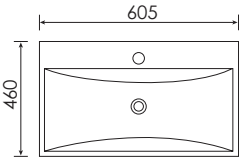
APOLLO 60 Ceramic basin size: 605x460x165 mm
