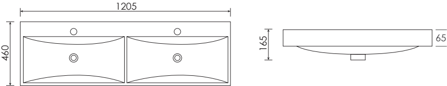
APOLLO 120D Ceramic basin size: 1205x460x165mm
