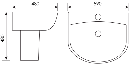
DIONE-59SP Semi-pedestal basin Size: 590x480x480mm
