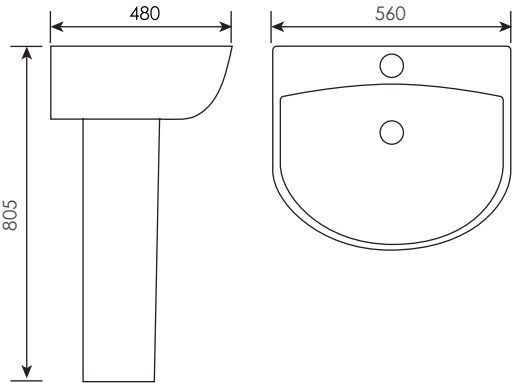
DIONE-59SP Pedestal basin Size: 560x480x805mm
