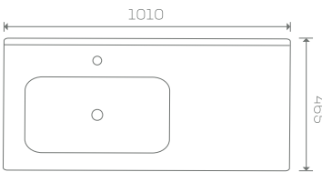
MONZA46 100L SIZE: 1010X465X170 MM
