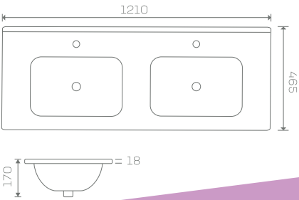
MONZA46 120D SIZE: 1210X465X170 MM
