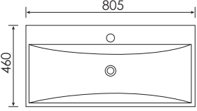
APOLLO 80 Ceramic basin size: 805x460x165 mm
