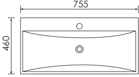
APOLLO 75 Ceramic basin size: 755x460x165 mm
