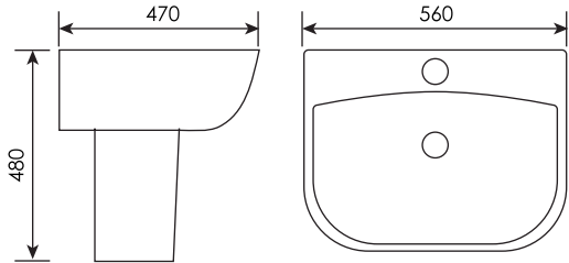
GLIDE-56SP Semi-pedestal basin Size: 560x470x480mm
