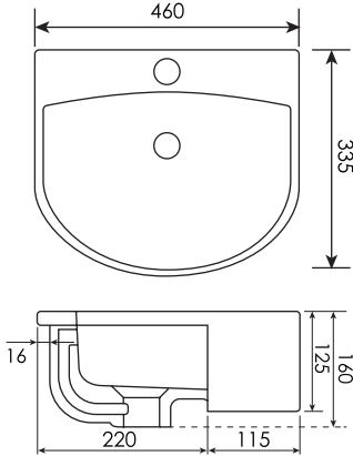
GLIDE-46SR Semi-recessed basin Size: 460x335x160mm
