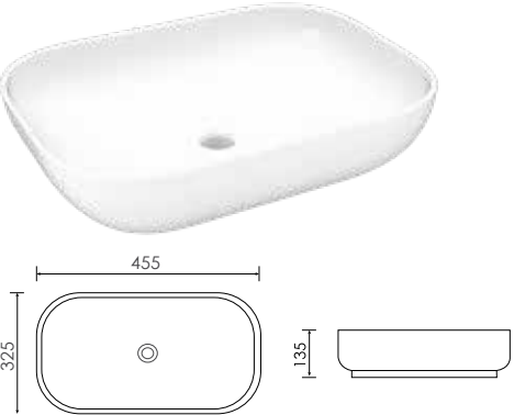
CBCLTA Ceramic basin size: 455x325x135mm
