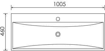
APOLLO 100 Ceramic basin size: 1005x460x165 mm
